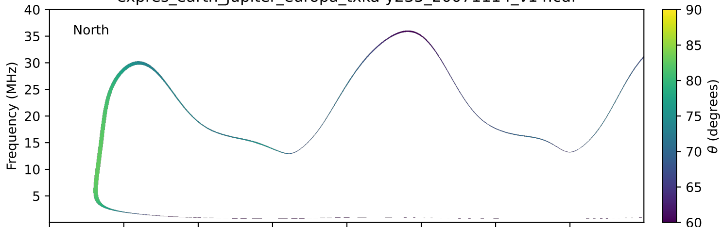
expres_earth_jupiter_europa_txka-y235_20071114_v14.cdf
