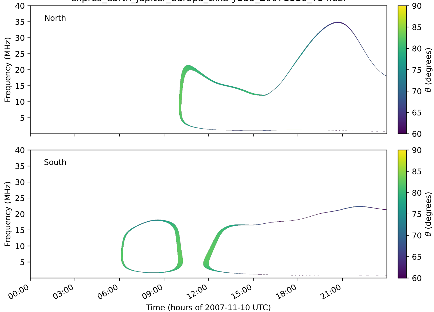
expres_earth_jupiter_europa_txka-y235_20071110_v14.cdf
