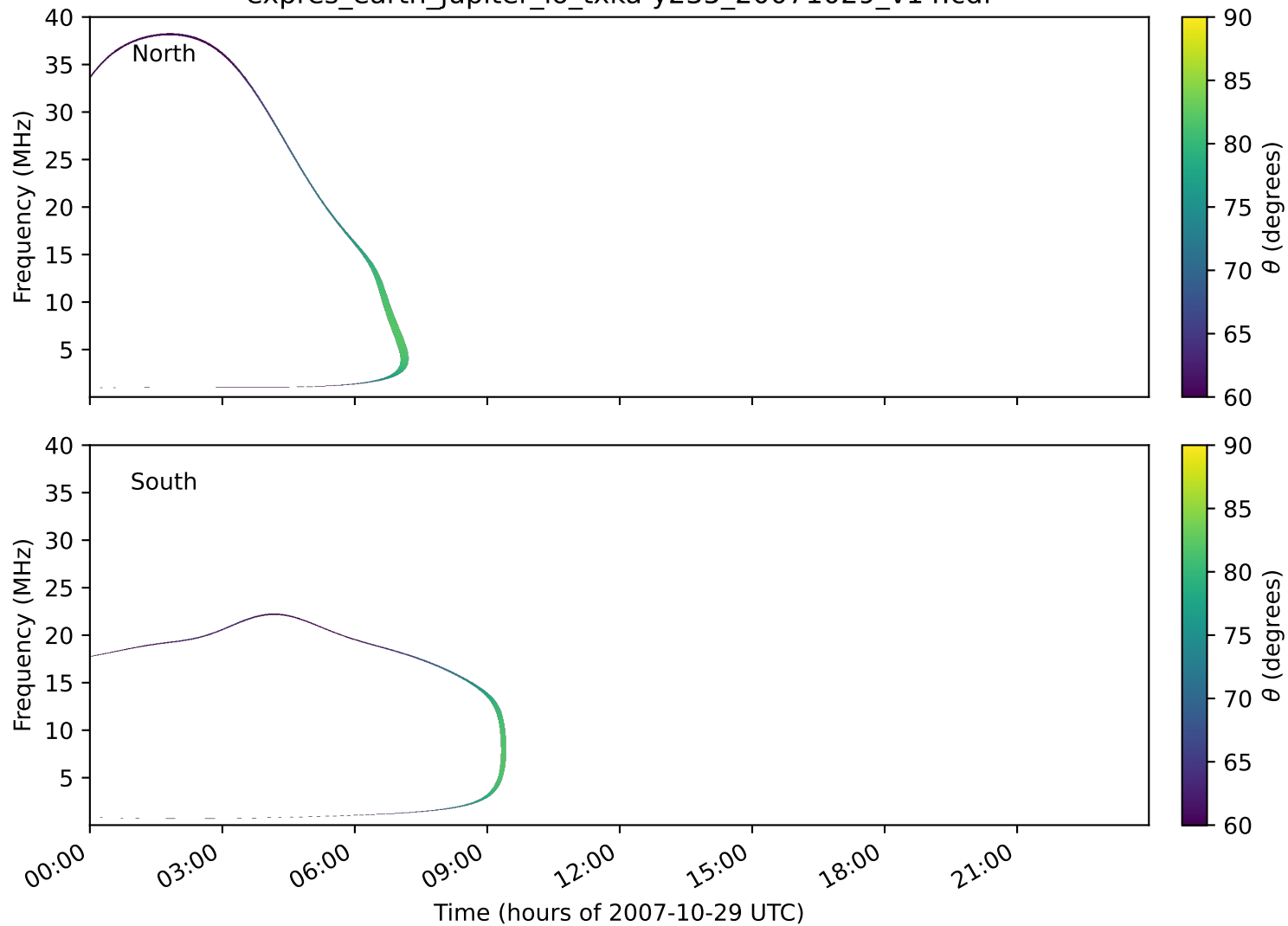
expres_earth_jupiter_io_txka-y235_20071029_v14.cdf
