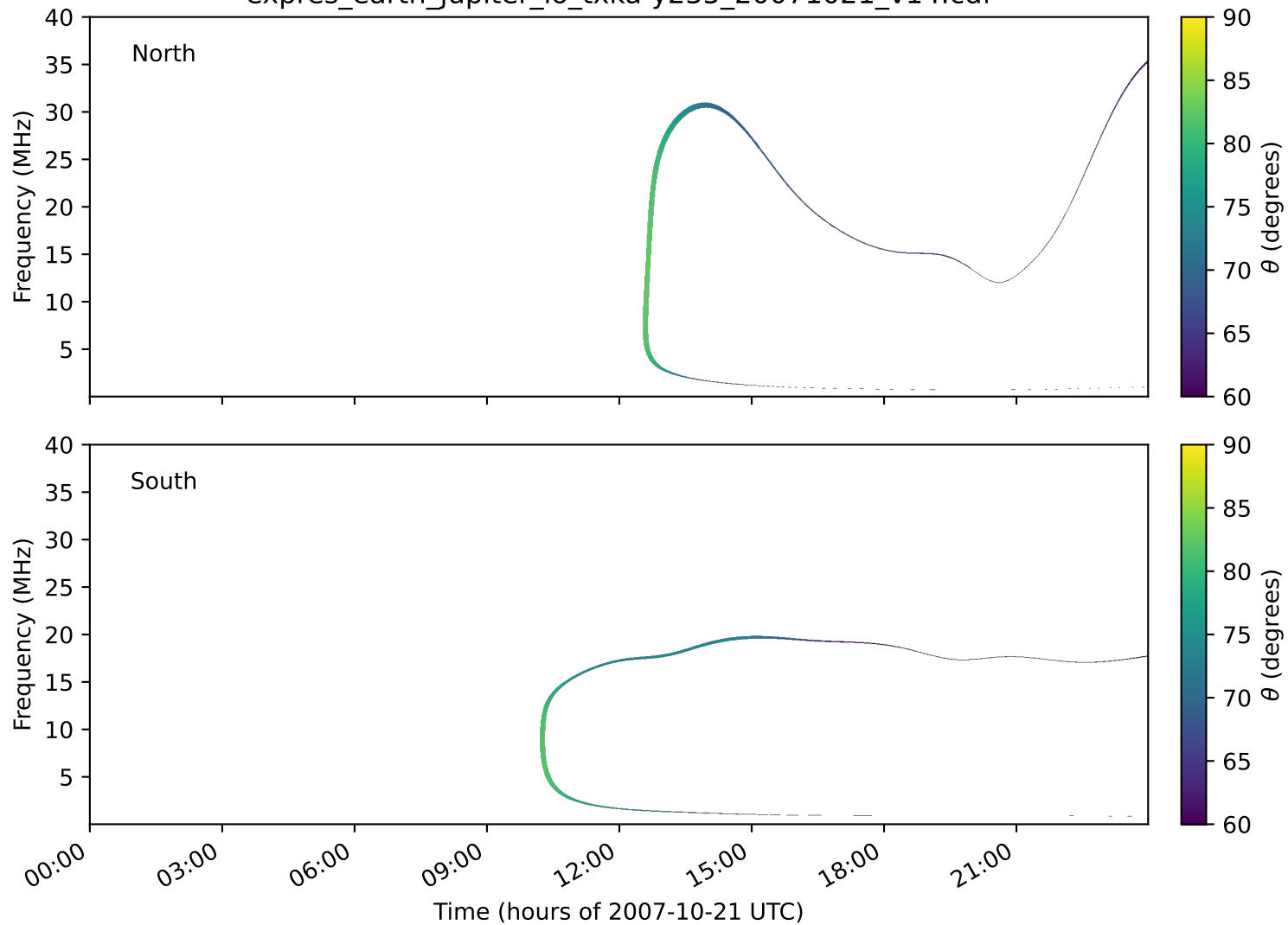
expres_earth_jupiter_io_txka-y235_20071021_v14.cdf
