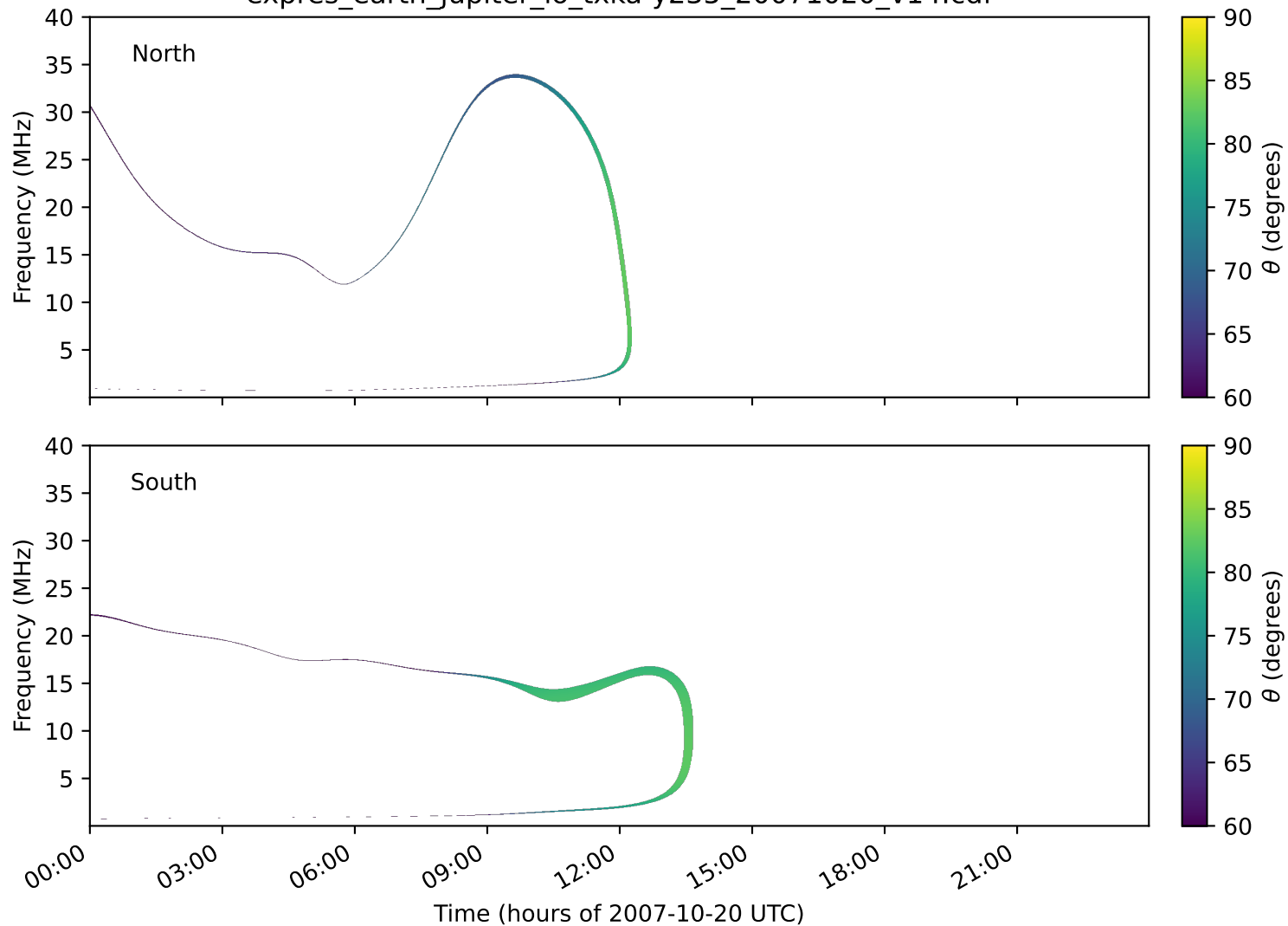
expres_earth_jupiter_io_txka-y235_20071020_v14.cdf
