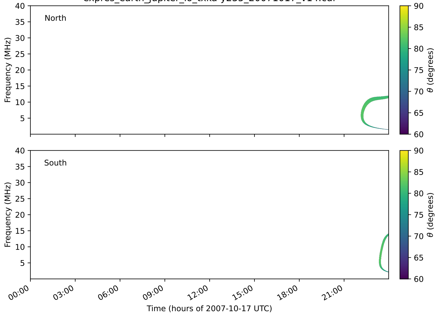
expres_earth_jupiter_io_txka-y235_20071017_v14.cdf
