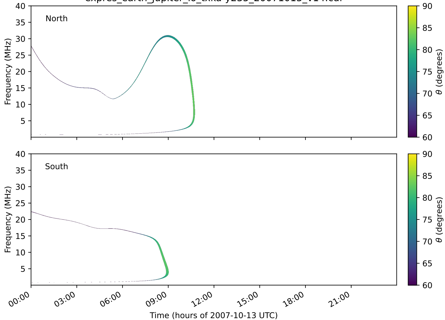
expres_earth_jupiter_io_txka-y235_20071013_v14.cdf
