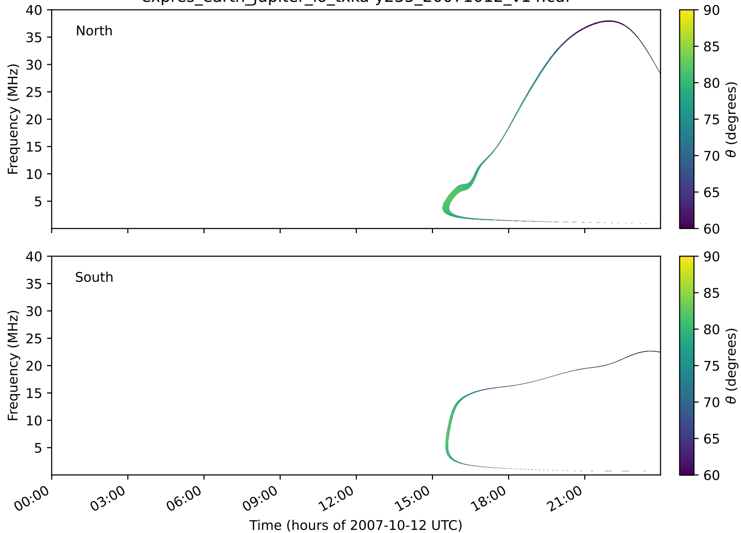
expres_earth_jupiter_io_txka-y235_20071012_v14.cdf
