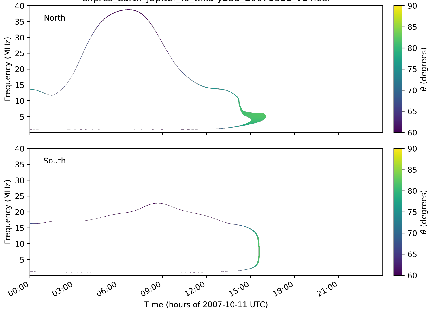
expres_earth_jupiter_io_txka-y235_20071011_v14.cdf
