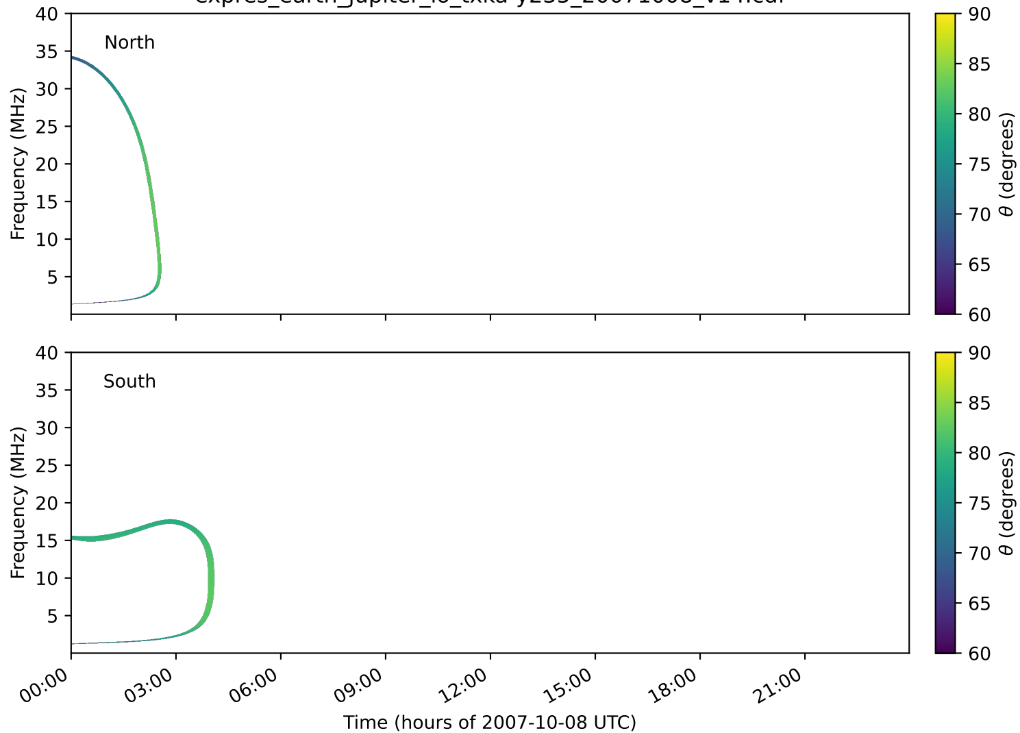
expres_earth_jupiter_io_txka-y235_20071008_v14.cdf
