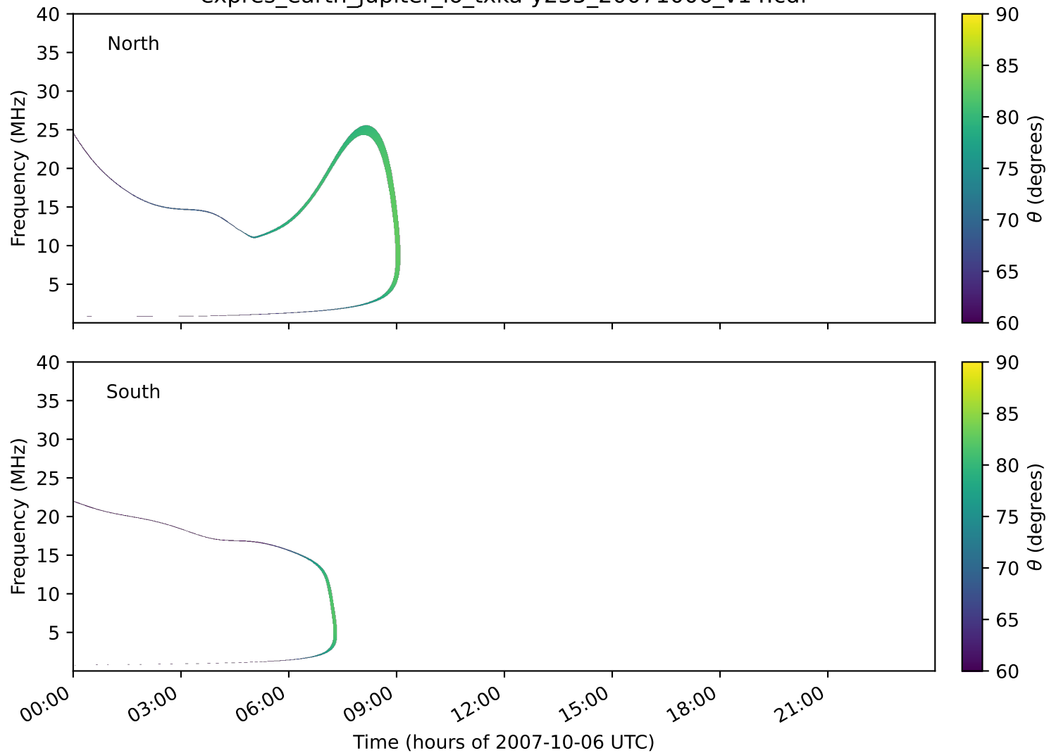
expres_earth_jupiter_io_txka-y235_20071006_v14.cdf
