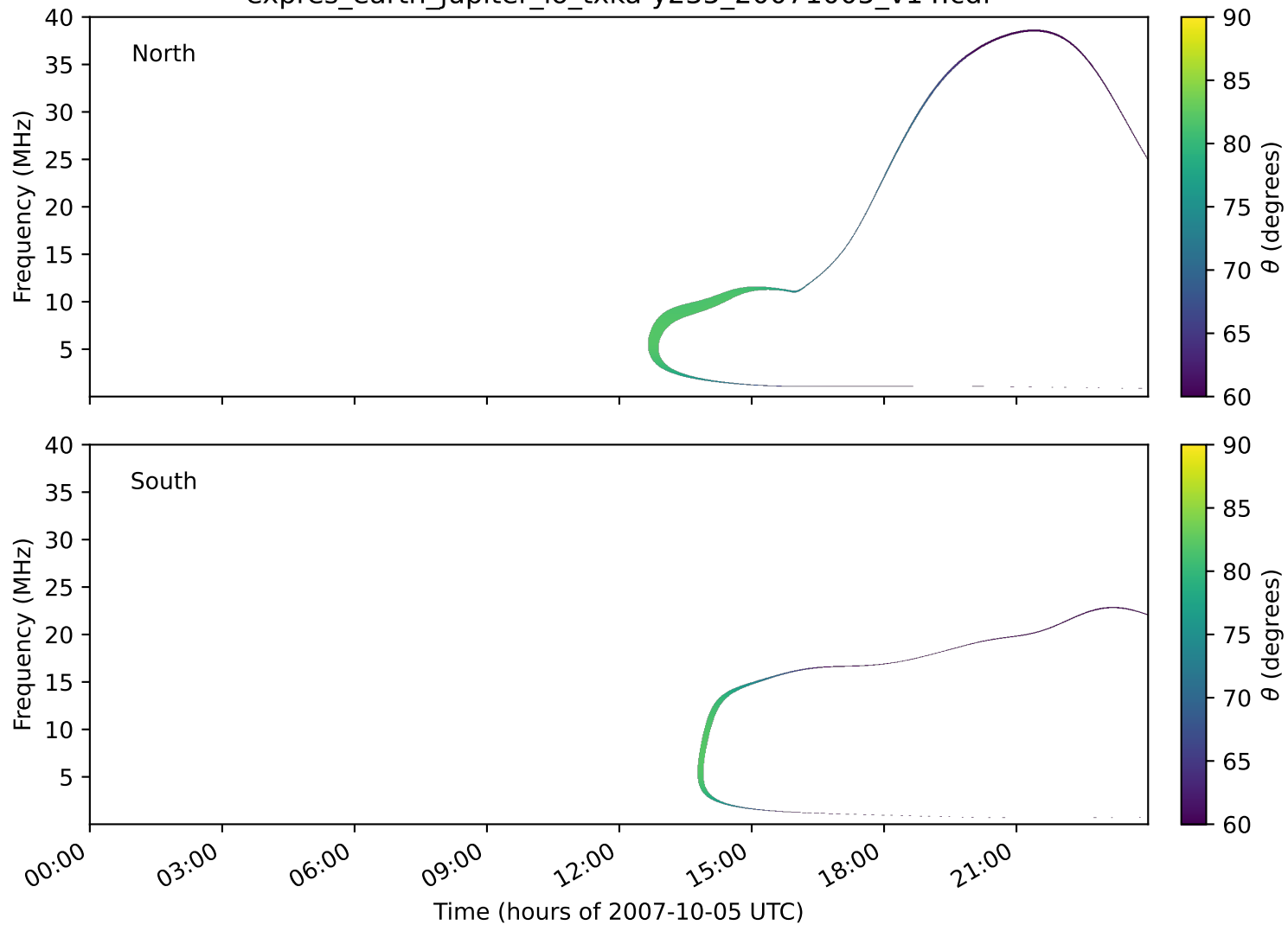
expres_earth_jupiter_io_txka-y235_20071005_v14.cdf
