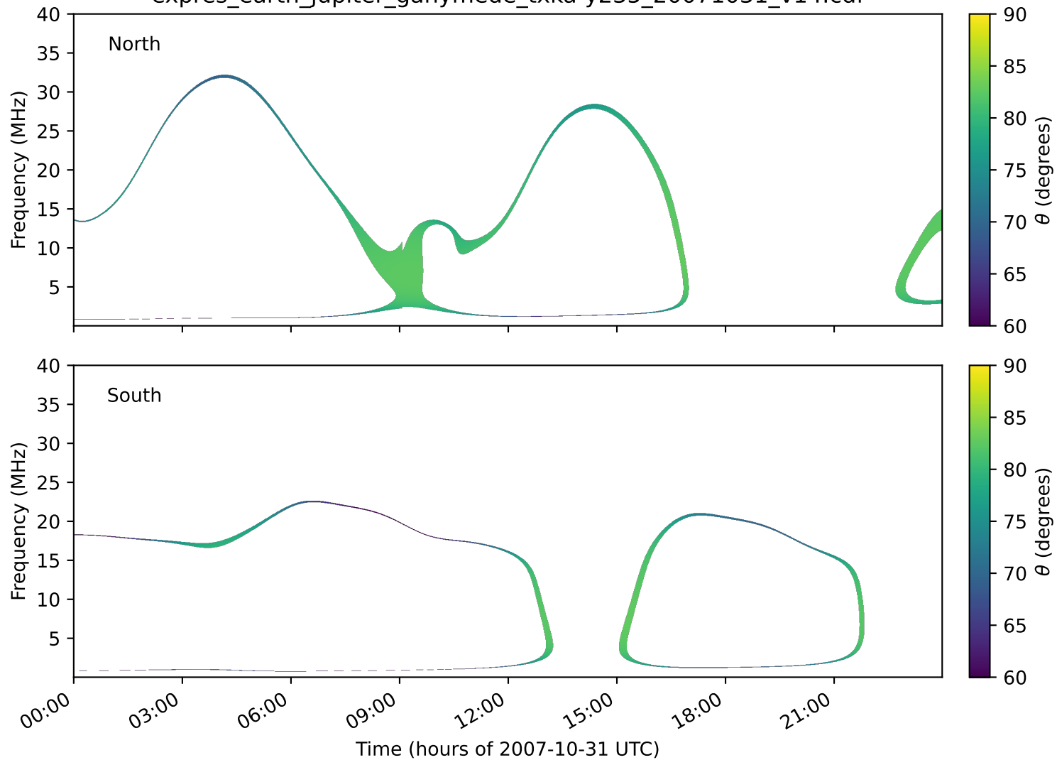
expres_earth_jupiter_ganymede_txka-y235_20071031_v14.cdf
