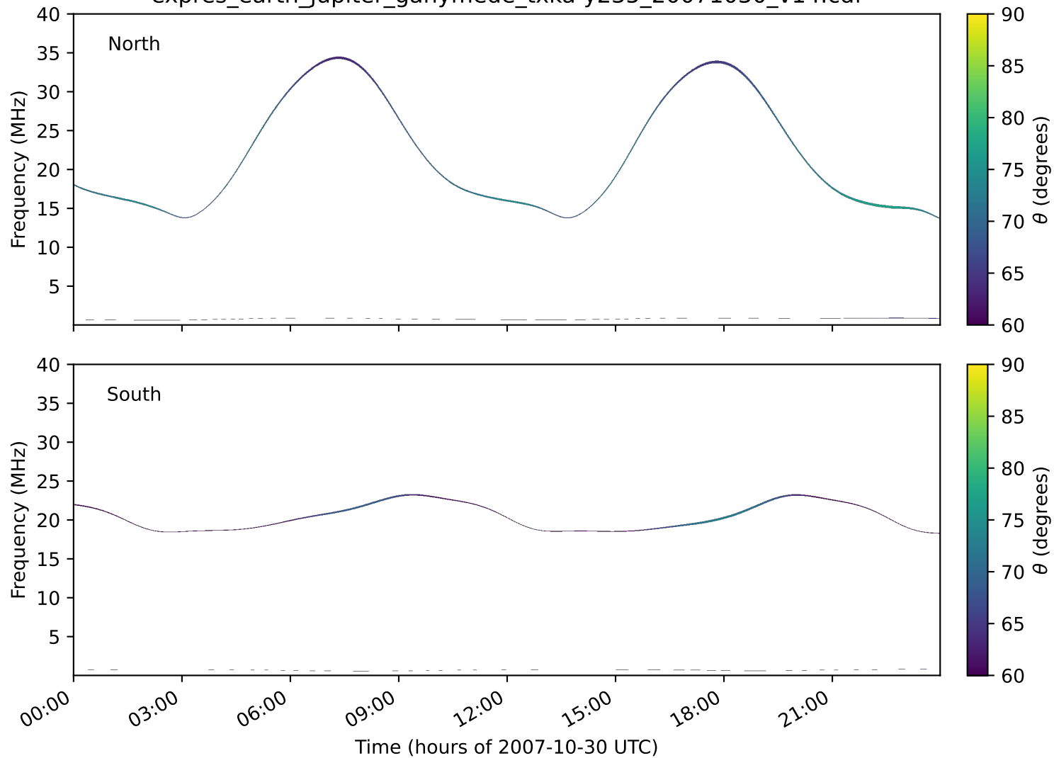
expres_earth_jupiter_ganymede_txka-y235_20071030_v14.cdf
