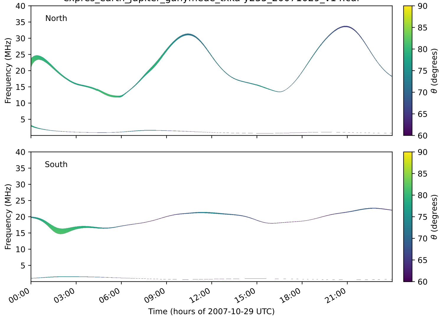
expres_earth_jupiter_ganymede_txka-y235_20071029_v14.cdf
