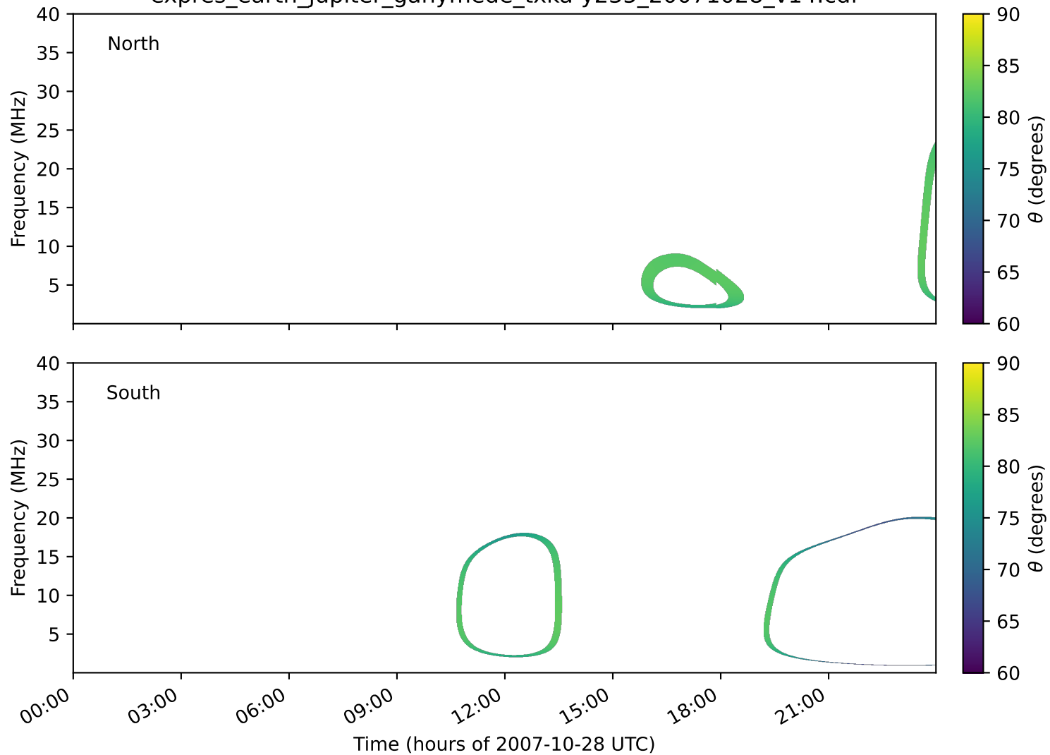
expres_earth_jupiter_ganymede_txka-y235_20071028_v14.cdf
