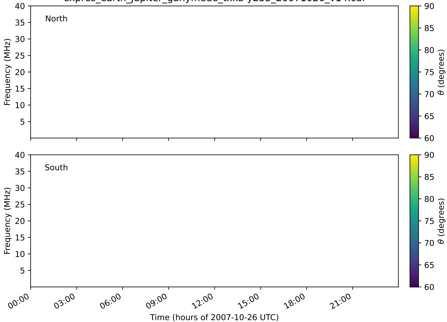
expres_earth_jupiter_ganymede_txka-y235_20071026_v14.cdf
