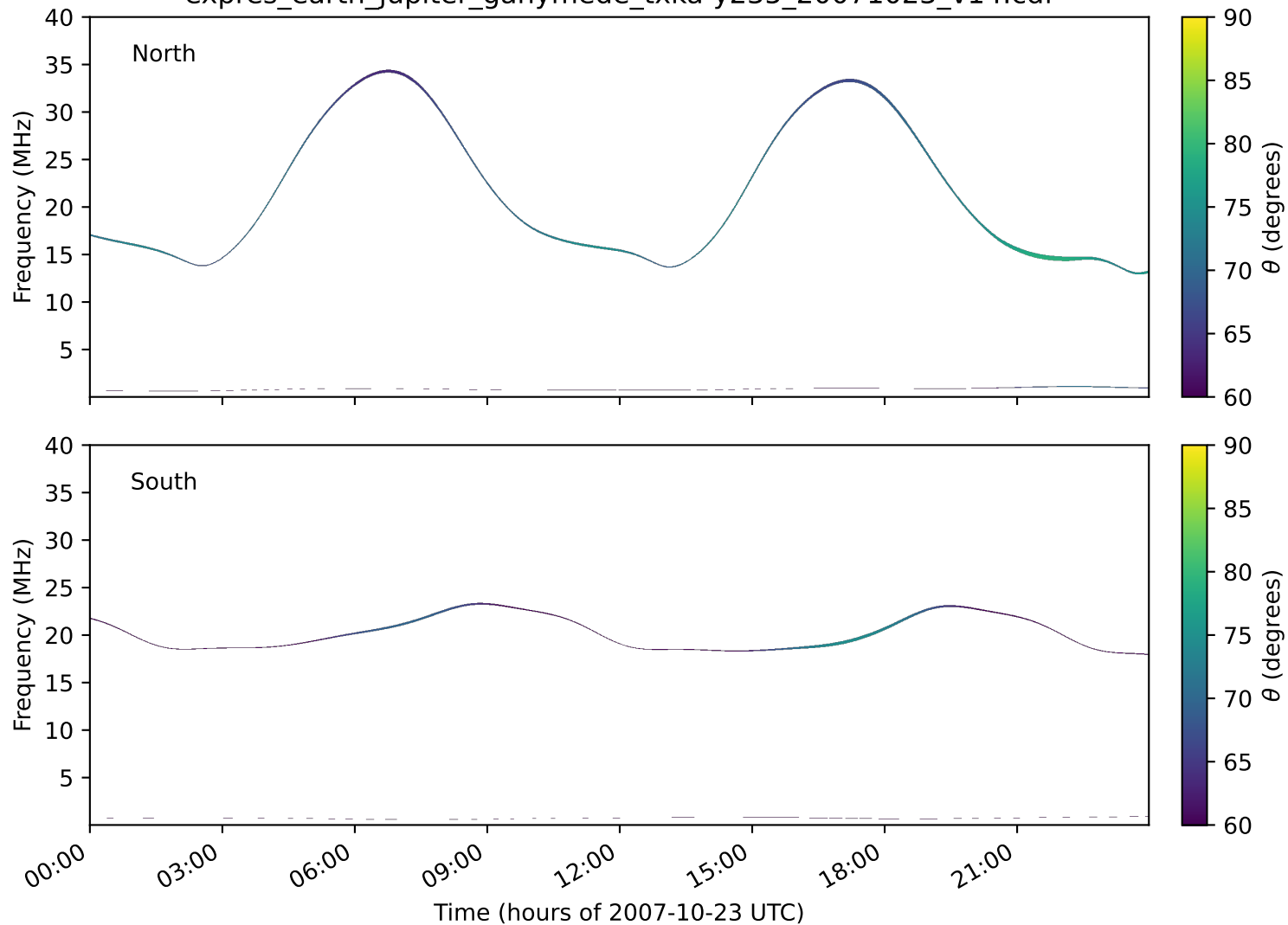
expres_earth_jupiter_ganymede_txka-y235_20071023_v14.cdf
