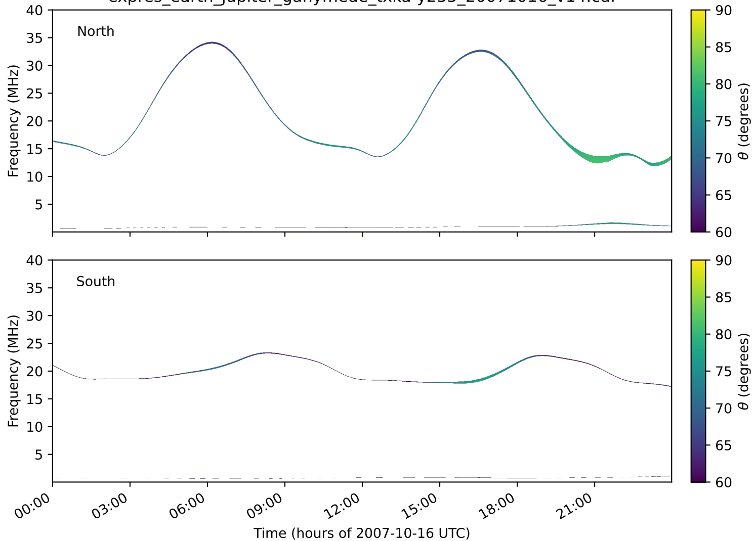
expres_earth_jupiter_ganymede_txka-y235_20071016_v14.cdf
