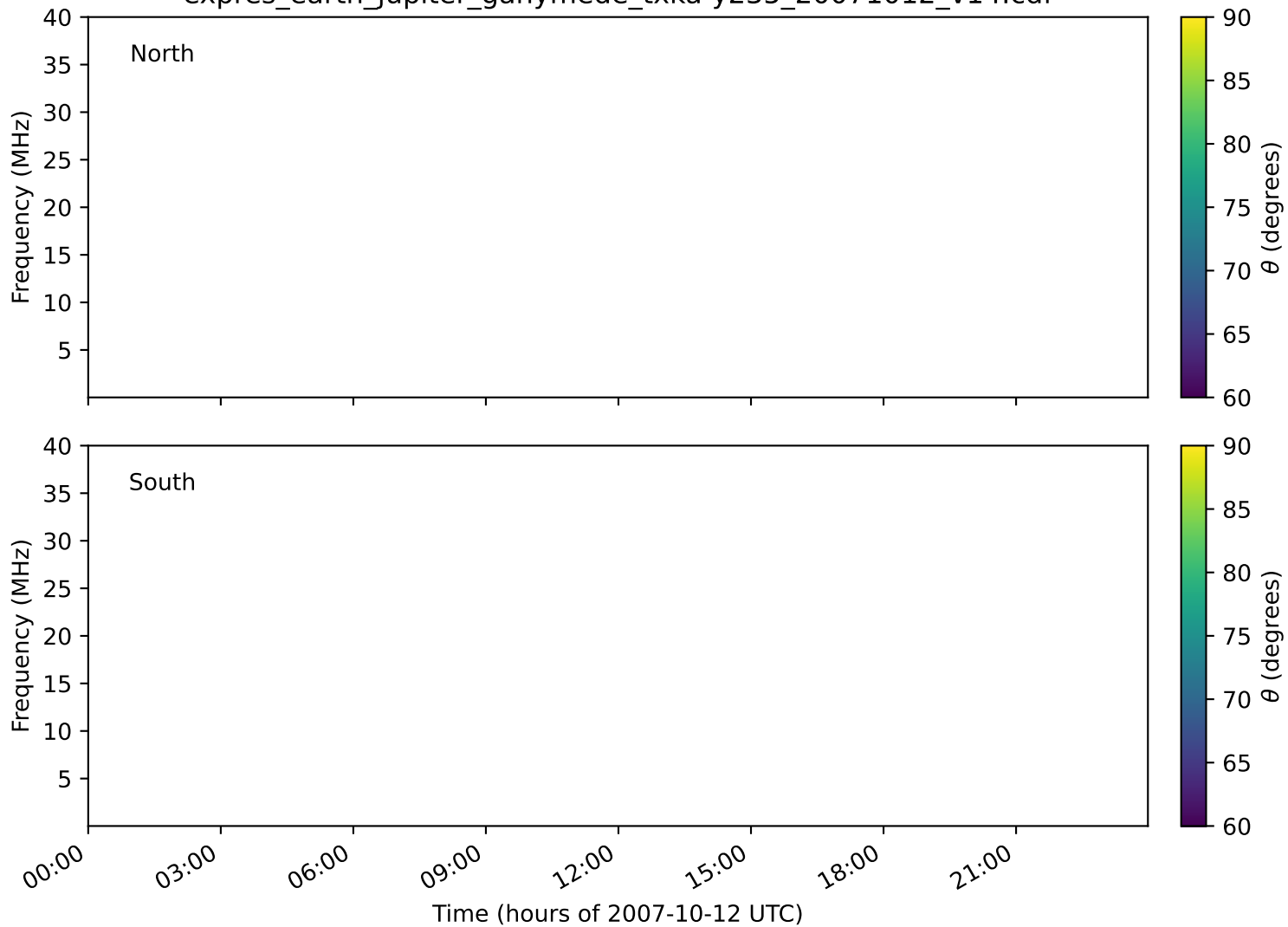
expres_earth_jupiter_ganymede_txka-y235_20071012_v14.cdf
