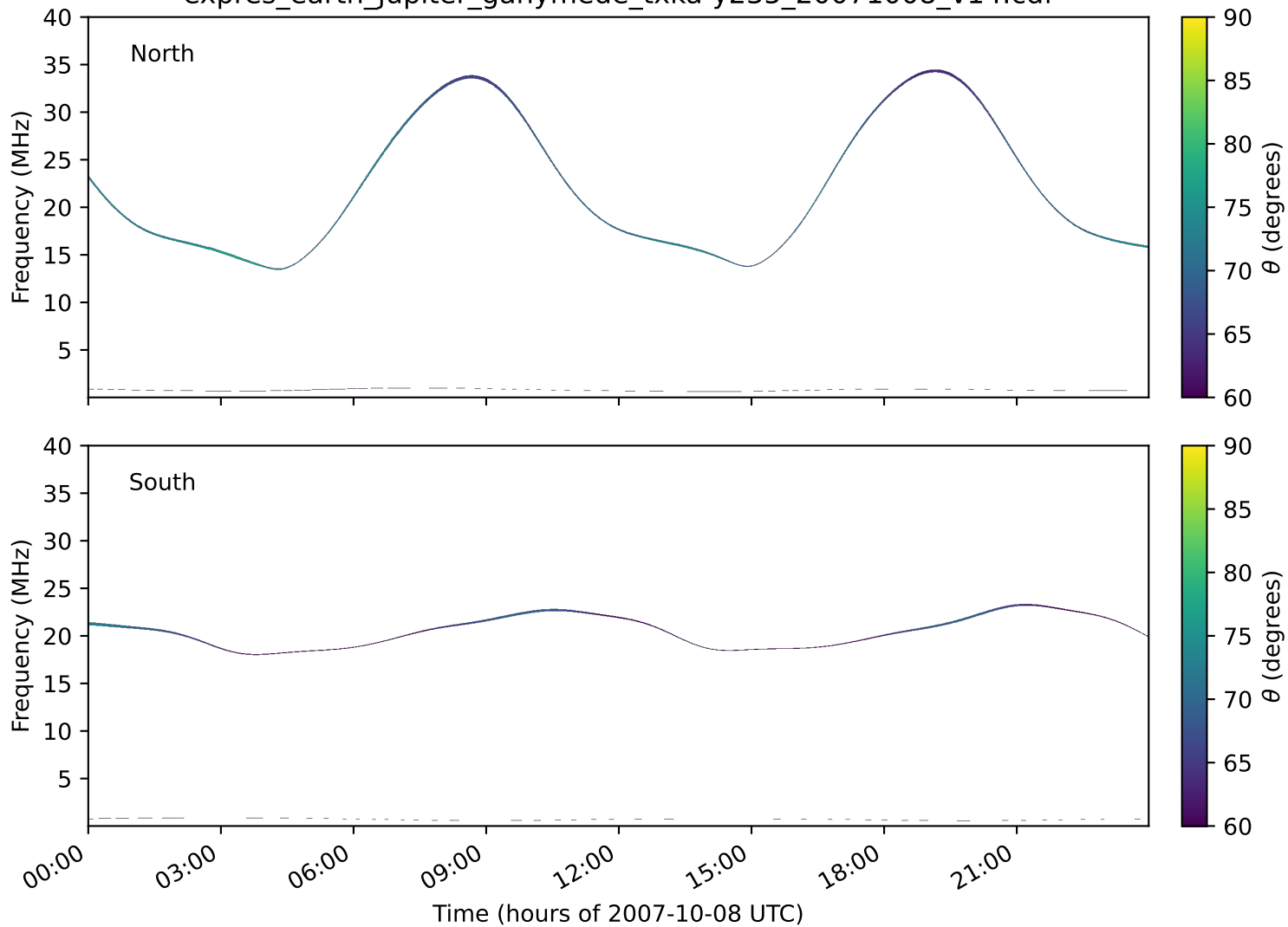
expres_earth_jupiter_ganymede_txka-y235_20071008_v14.cdf
