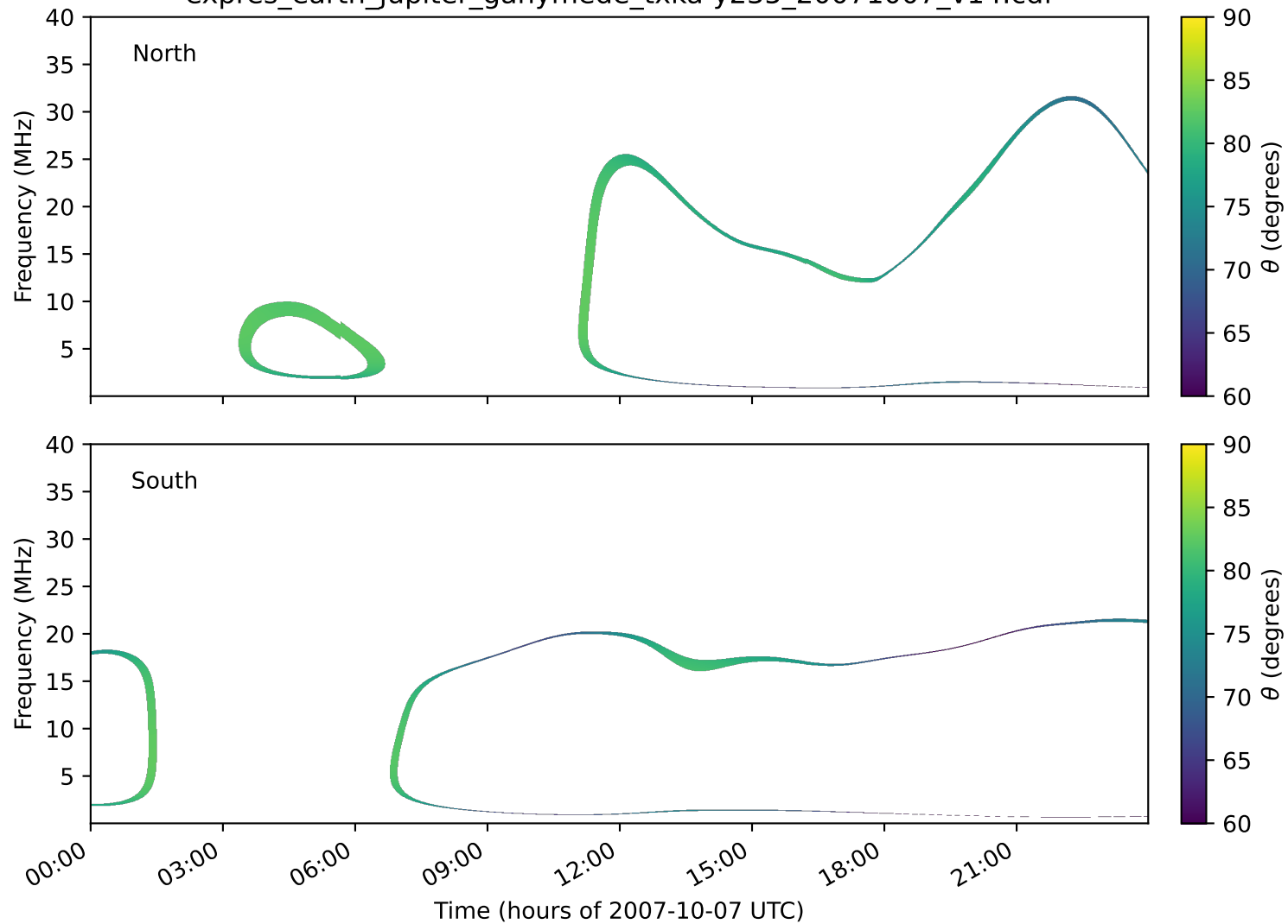
expres_earth_jupiter_ganymede_txka-y235_20071007_v14.cdf
