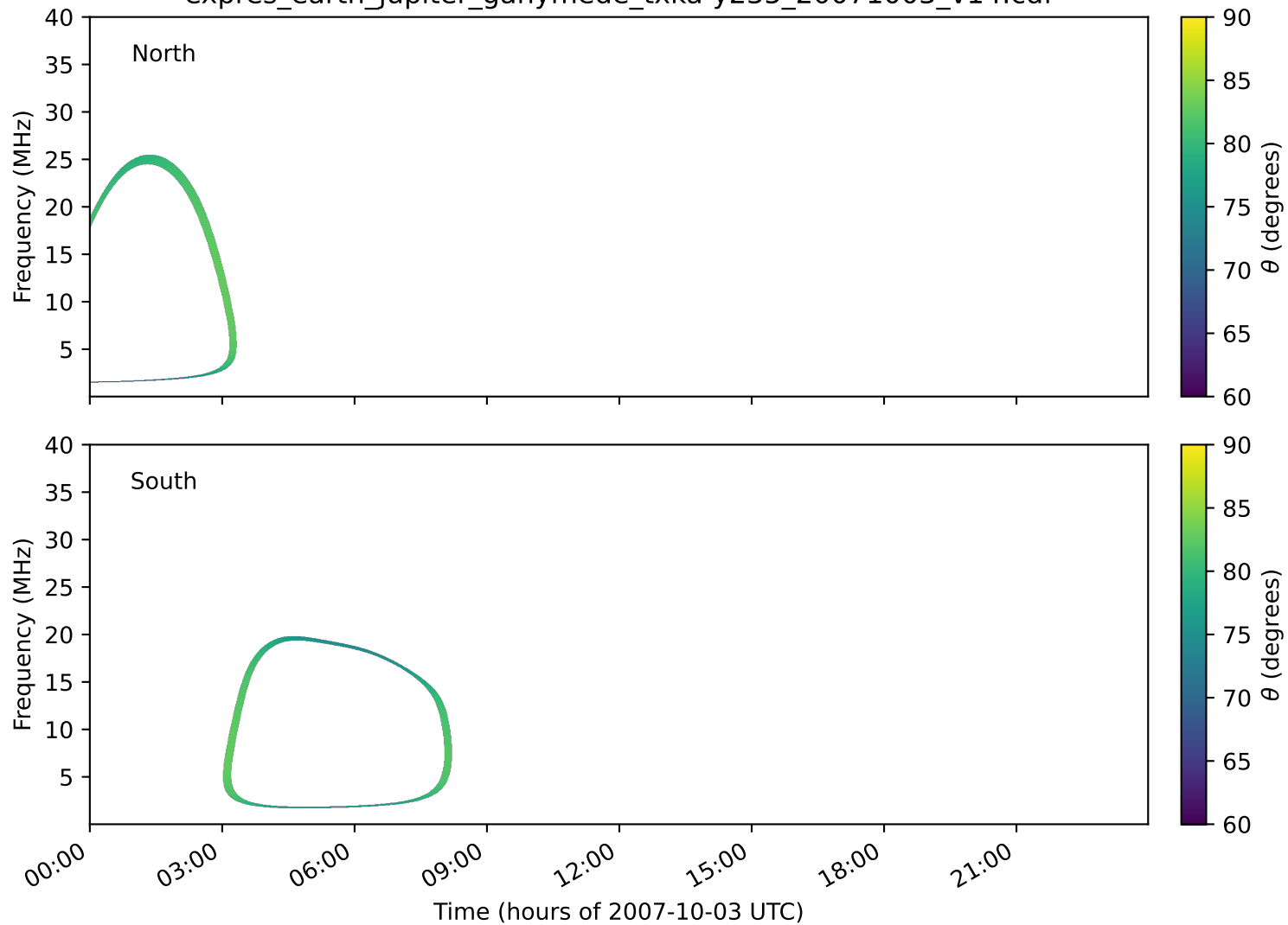
expres_earth_jupiter_ganymede_txka-y235_20071003_v14.cdf
