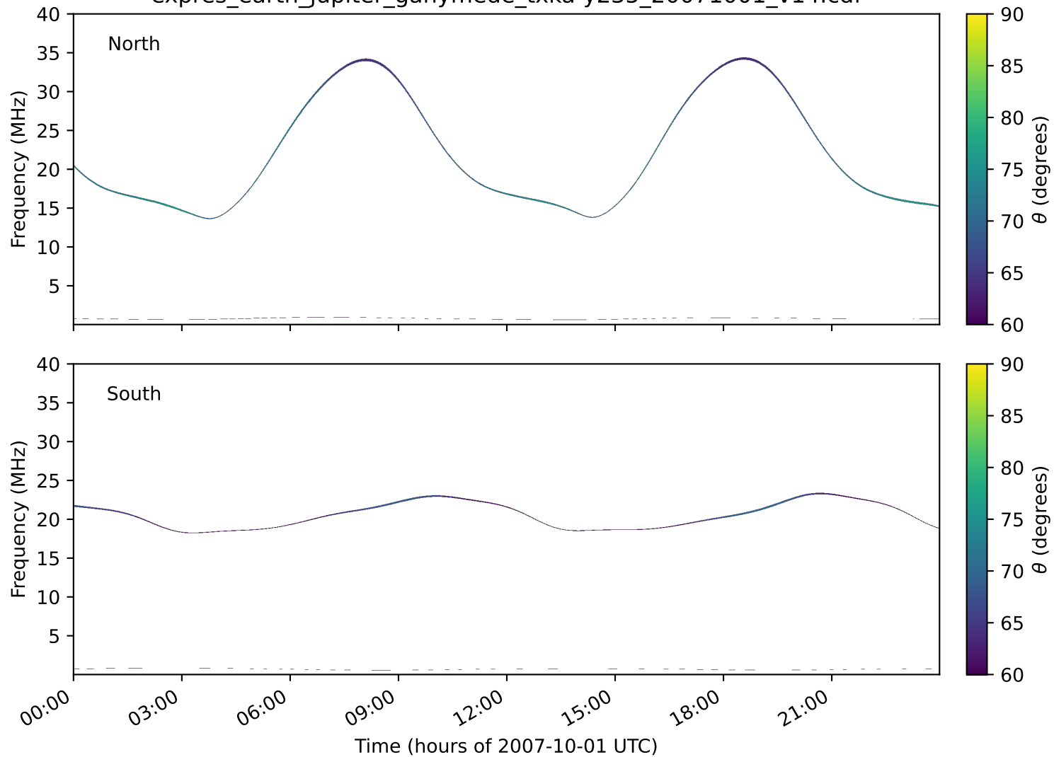
expres_earth_jupiter_ganymede_txka-y235_20071001_v14.cdf
