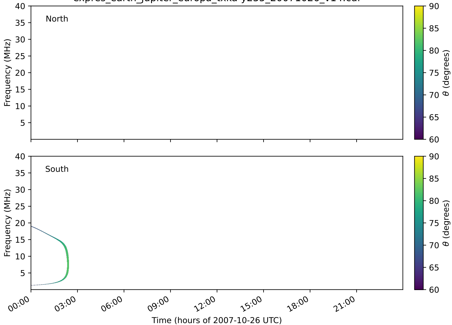
expres_earth_jupiter_europa_txka-y235_20071026_v14.cdf
