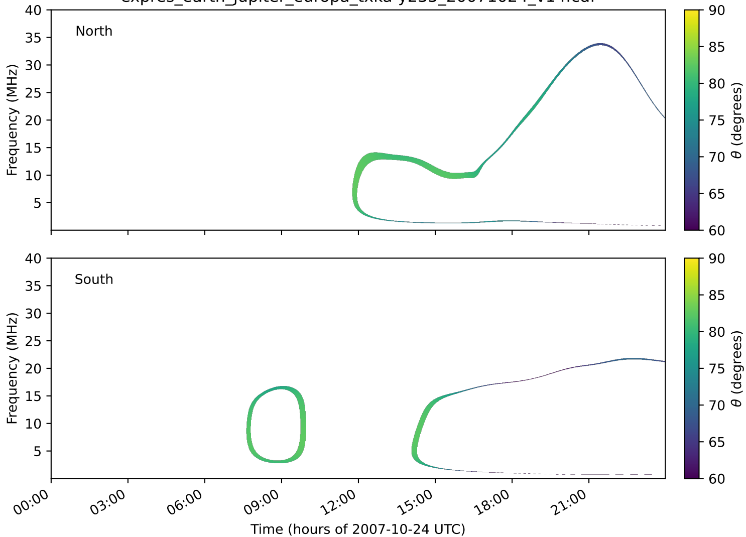
expres_earth_jupiter_europa_txka-y235_20071024_v14.cdf
