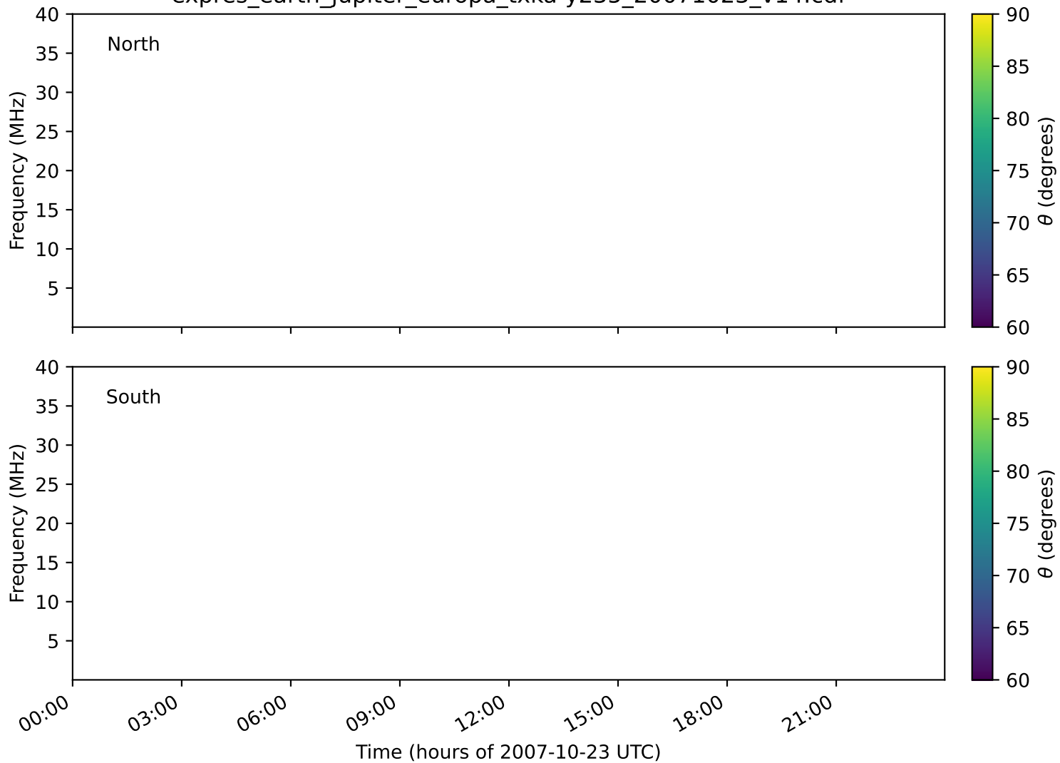
expres_earth_jupiter_europa_txka-y235_20071023_v14.cdf
