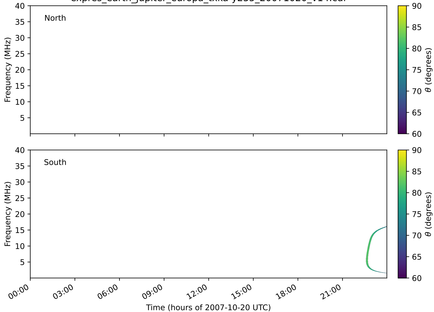
expres_earth_jupiter_europa_txka-y235_20071020_v14.cdf
