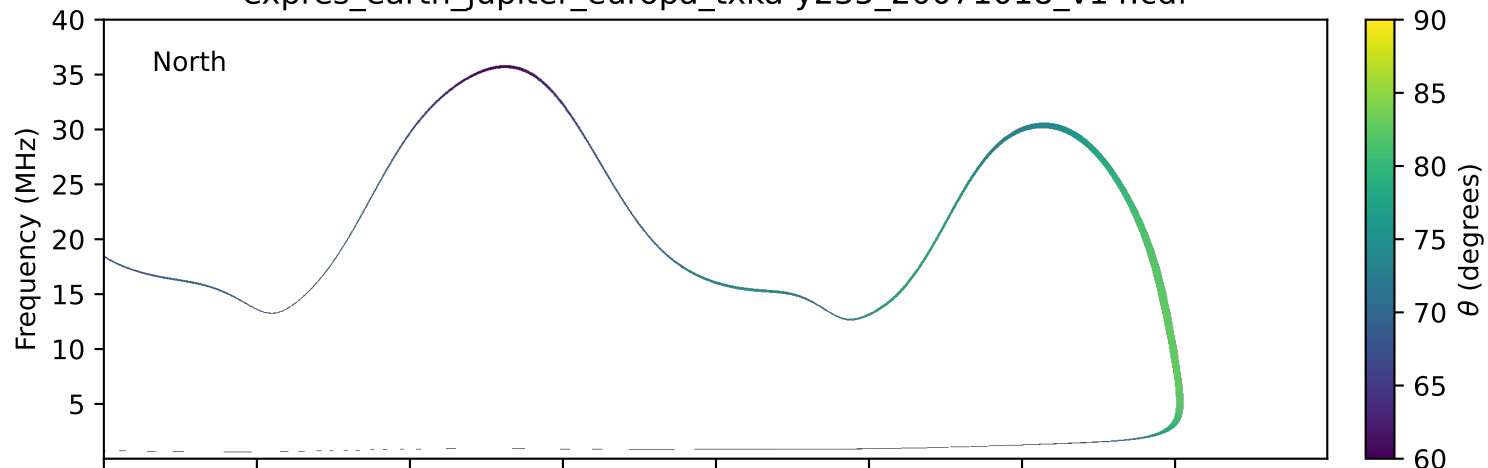
expres_earth_jupiter_europa_txka-y235_20071018_v14.cdf
