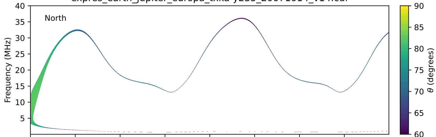
expres_earth_jupiter_europa_txka-y235_20071014_v14.cdf
