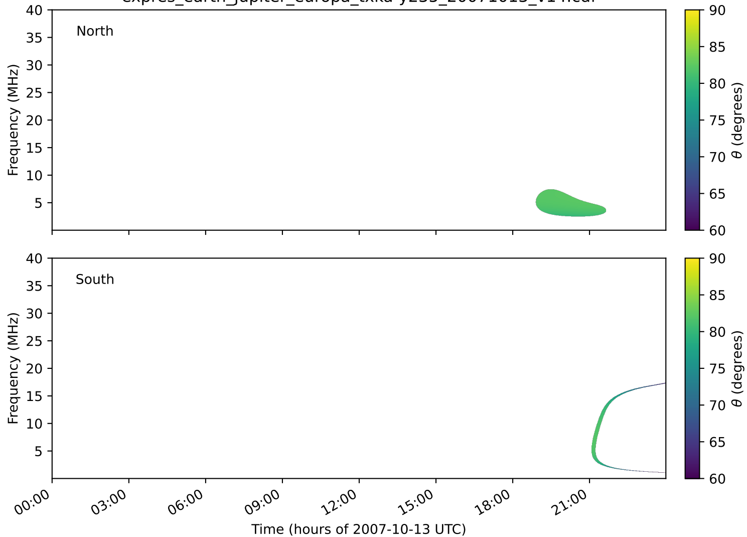
expres_earth_jupiter_europa_txka-y235_20071013_v14.cdf
