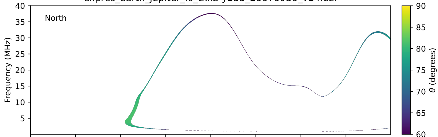
expres_earth_jupiter_io_txka-y235_20070930_v14.cdf
