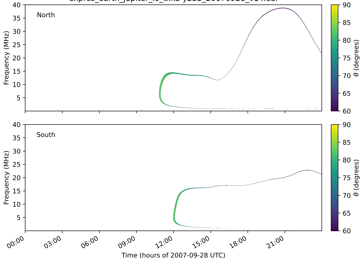
expres_earth_jupiter_io_txka-y235_20070928_v14.cdf
