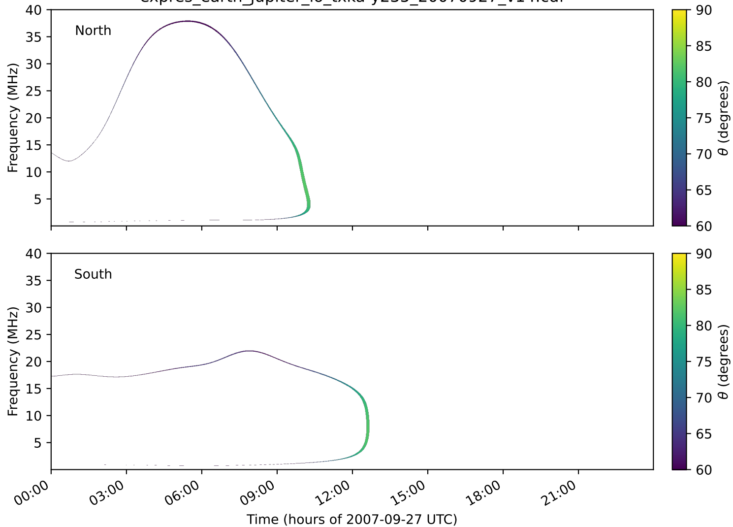
expres_earth_jupiter_io_txka-y235_20070927_v14.cdf
