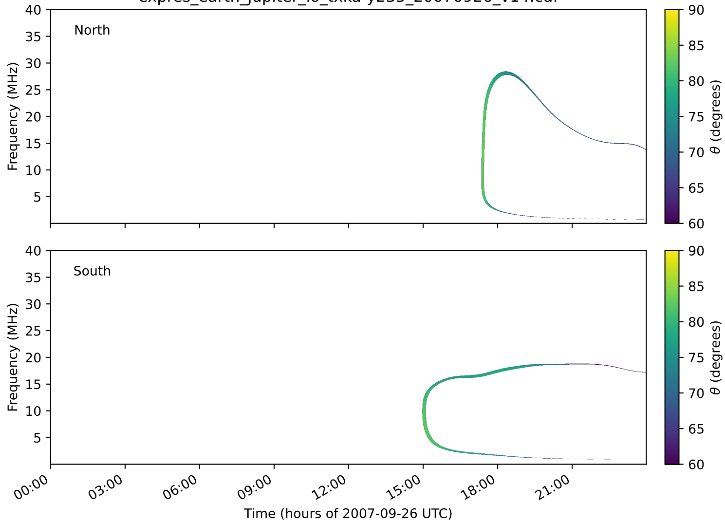
expres_earth_jupiter_io_txka-y235_20070926_v14.cdf
