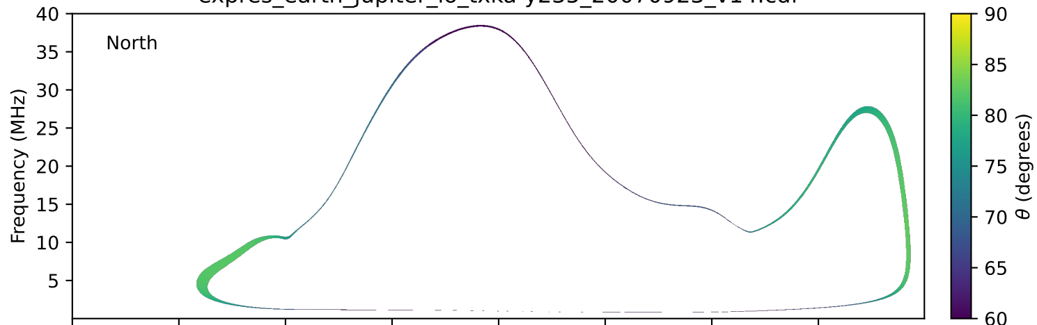
expres_earth_jupiter_io_txka-y235_20070923_v14.cdf
