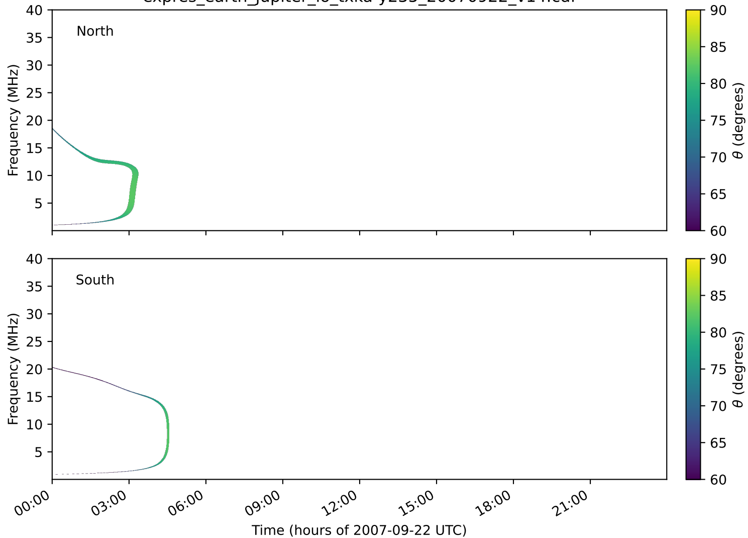
expres_earth_jupiter_io_txka-y235_20070922_v14.cdf
