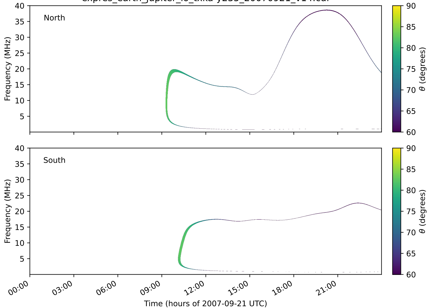
expres_earth_jupiter_io_txka-y235_20070921_v14.cdf
