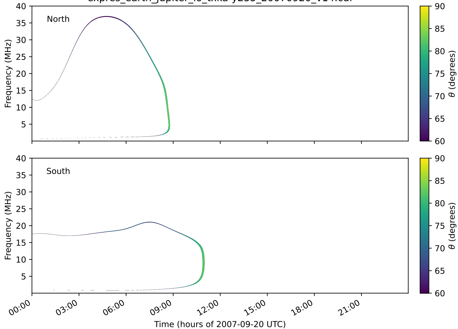
expres_earth_jupiter_io_txka-y235_20070920_v14.cdf
