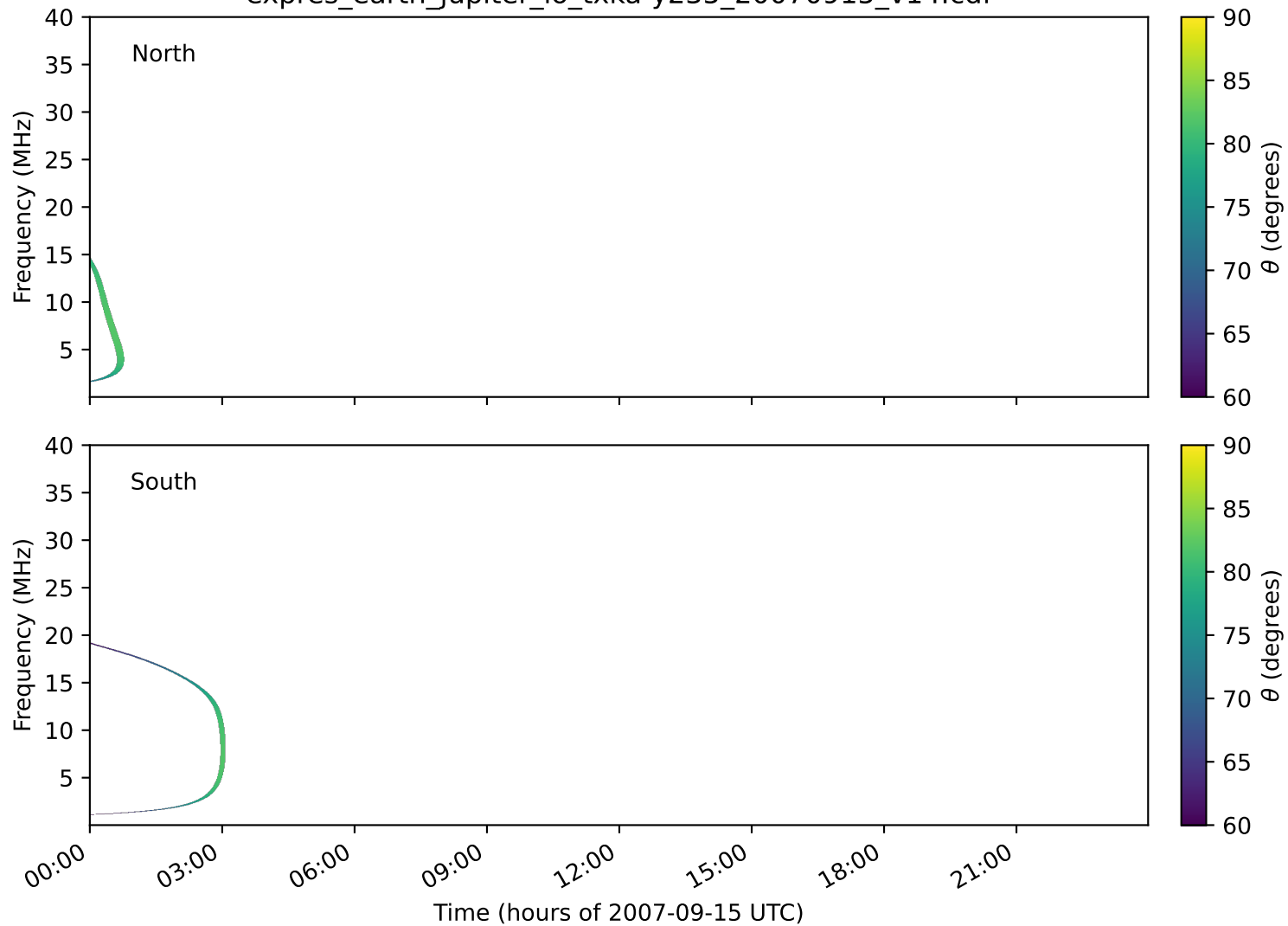
expres_earth_jupiter_io_txka-y235_20070915_v14.cdf
