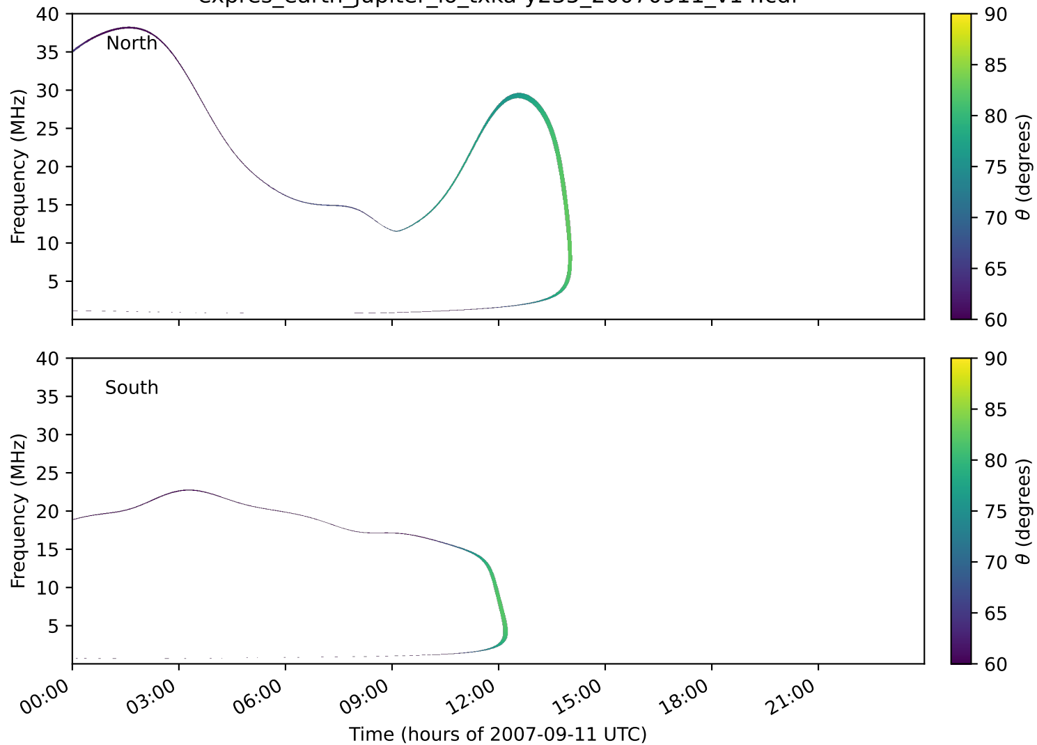
expres_earth_jupiter_io_txka-y235_20070911_v14.cdf
