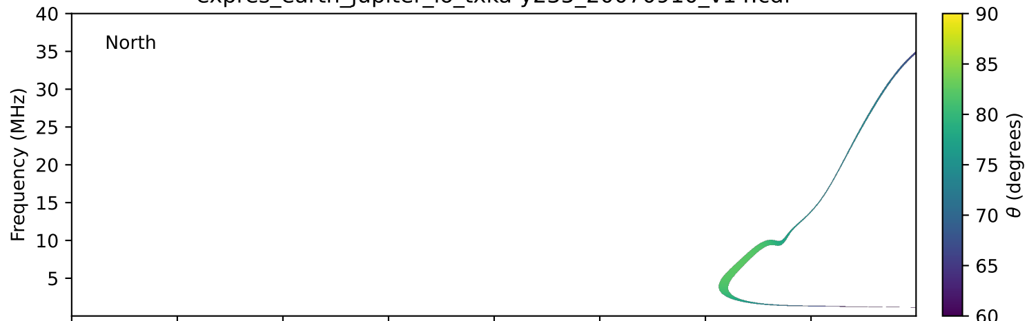
expres_earth_jupiter_io_txka-y235_20070910_v14.cdf
