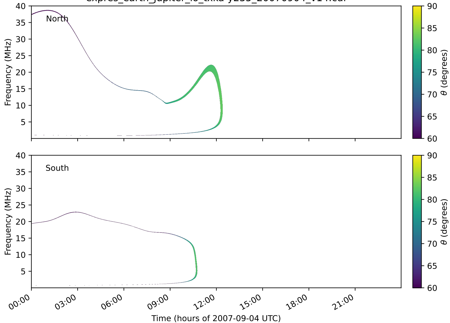
expres_earth_jupiter_io_txka-y235_20070904_v14.cdf
