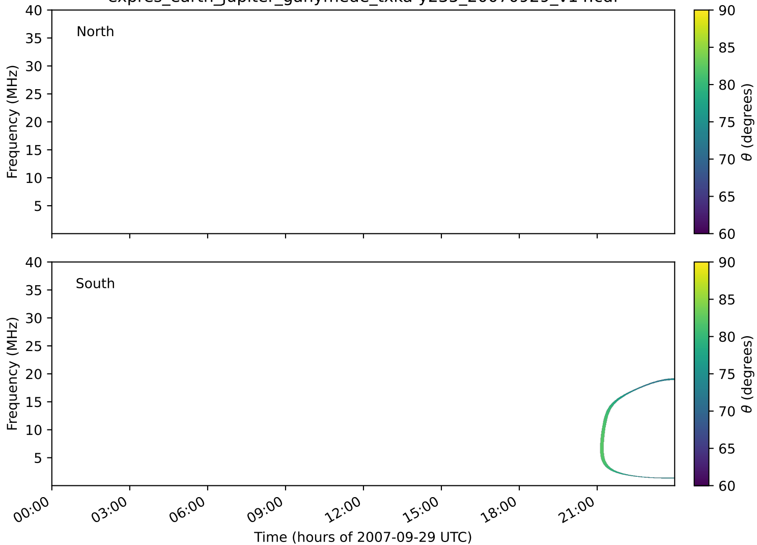
expres_earth_jupiter_ganymede_txka-y235_20070929_v14.cdf
