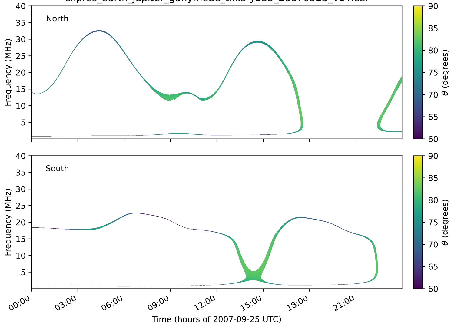
expres_earth_jupiter_ganymede_txka-y235_20070925_v14.cdf
