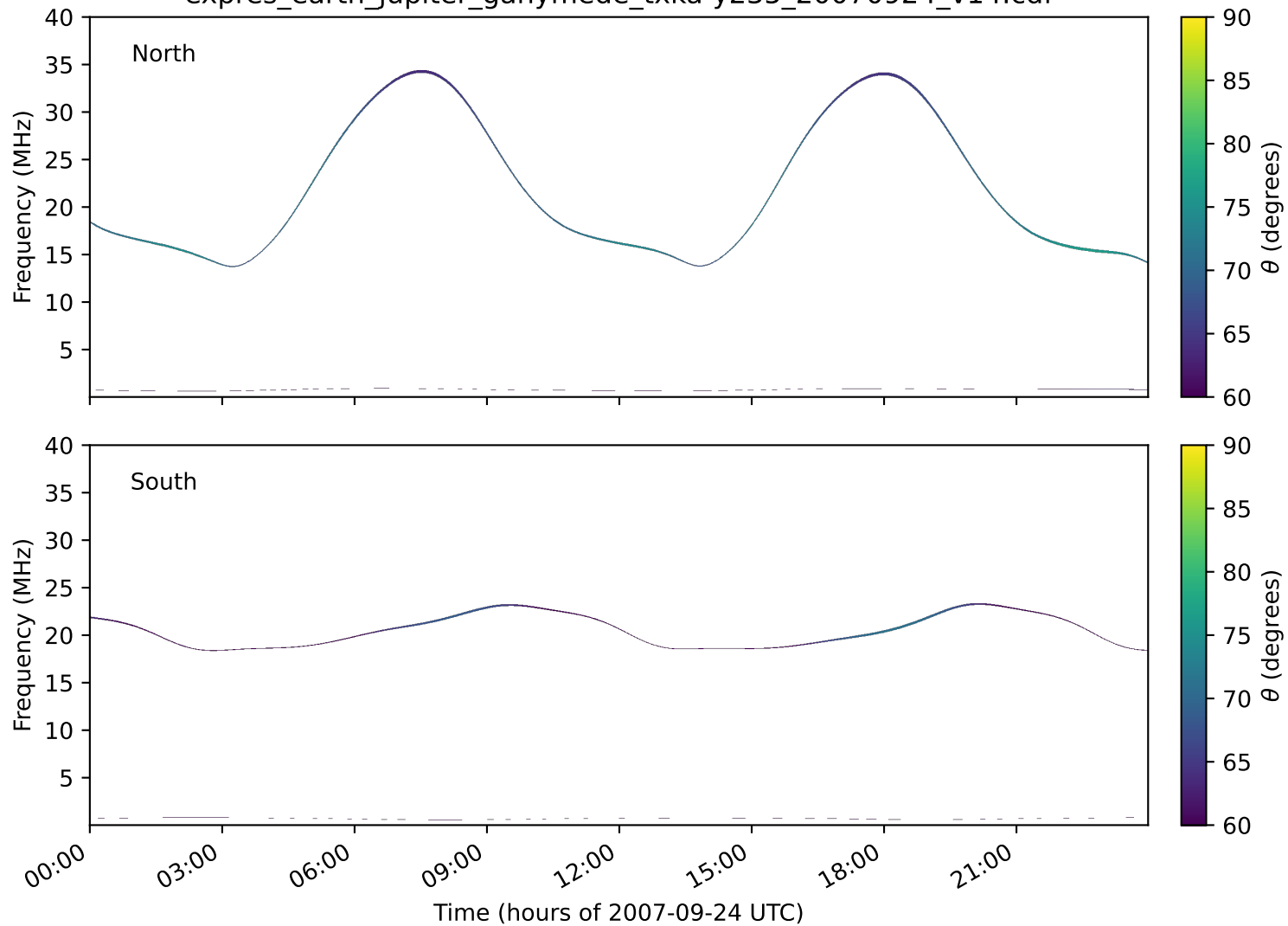
expres_earth_jupiter_ganymede_txka-y235_20070924_v14.cdf
