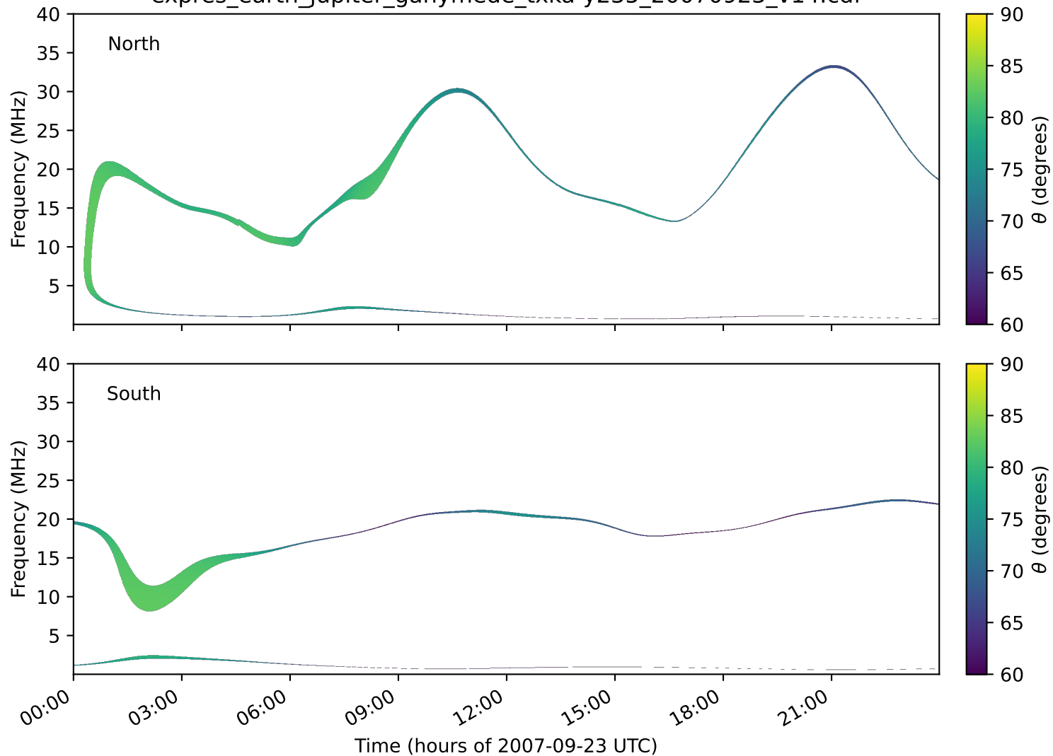
expres_earth_jupiter_ganymede_txka-y235_20070923_v14.cdf
