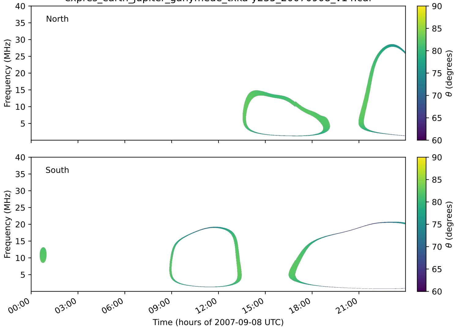
expres_earth_jupiter_ganymede_txka-y235_20070908_v14.cdf
