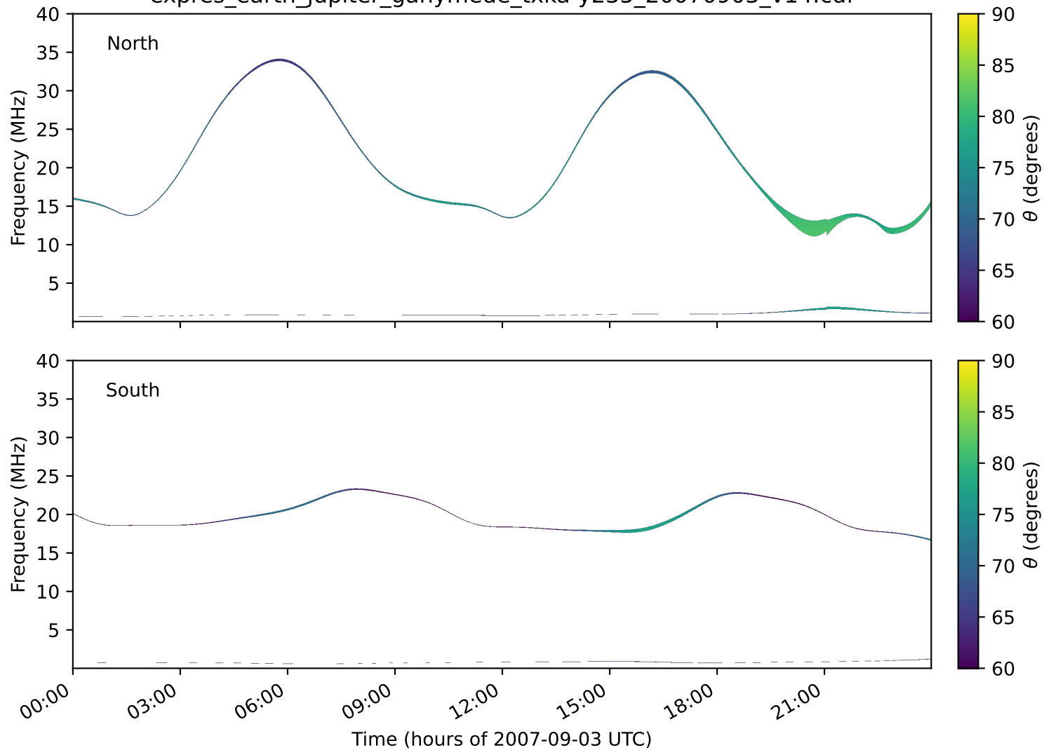
expres_earth_jupiter_ganymede_txka-y235_20070903_v14.cdf
