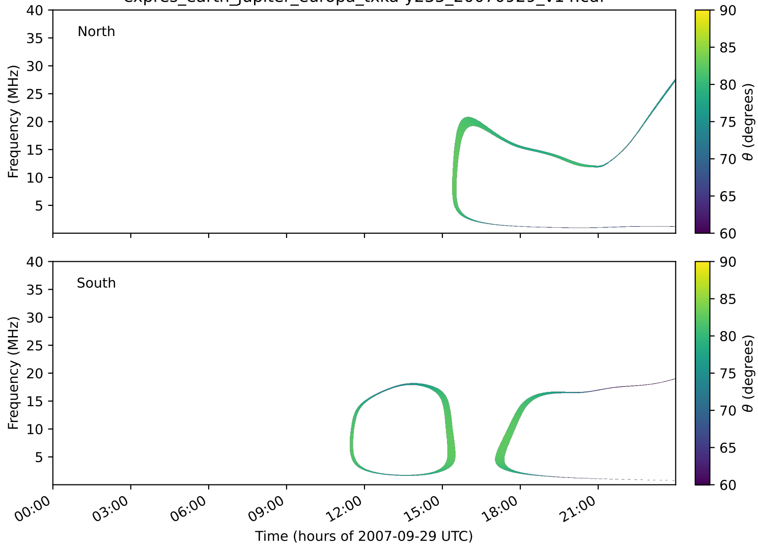
expres_earth_jupiter_europa_txka-y235_20070929_v14.cdf
